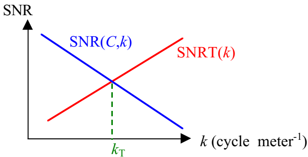
Figure 8b. The results of pre-existing, controlled experiments (human operators vs. patterns of varying spatial frequencies and contrasts on CRT screens) are combined with a model of the imaging process to derive an SNR Threshold (SNRT) for the Human Visual System (HVS). The objective is to discern Johnson bar patterns as a function of their spatial frequency k in the object plane. SNRT(k) is compared with SNR(C,k) , the SNR calculated for HVS observations of Johnson bar patterns with spatial frequency k , where C , the contrast, is set equal to the characteristic contrast of the targets in the
