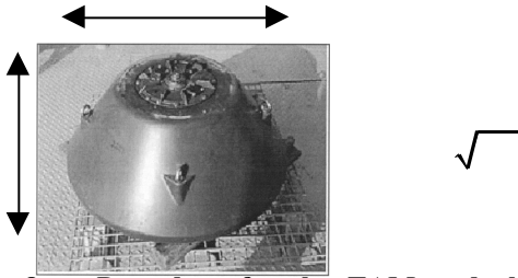
Figure 8a. Procedure for the TAM and the EO/ID problem. The target's critical dimension d_c and characteristic contrast C are determined.
